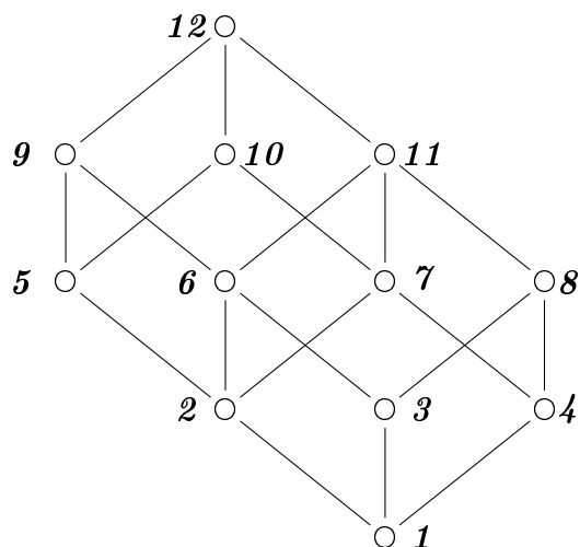
Figure 3: Factor lattice \mathcal{B}(G, M, I)/\frac{1}{2}E .
