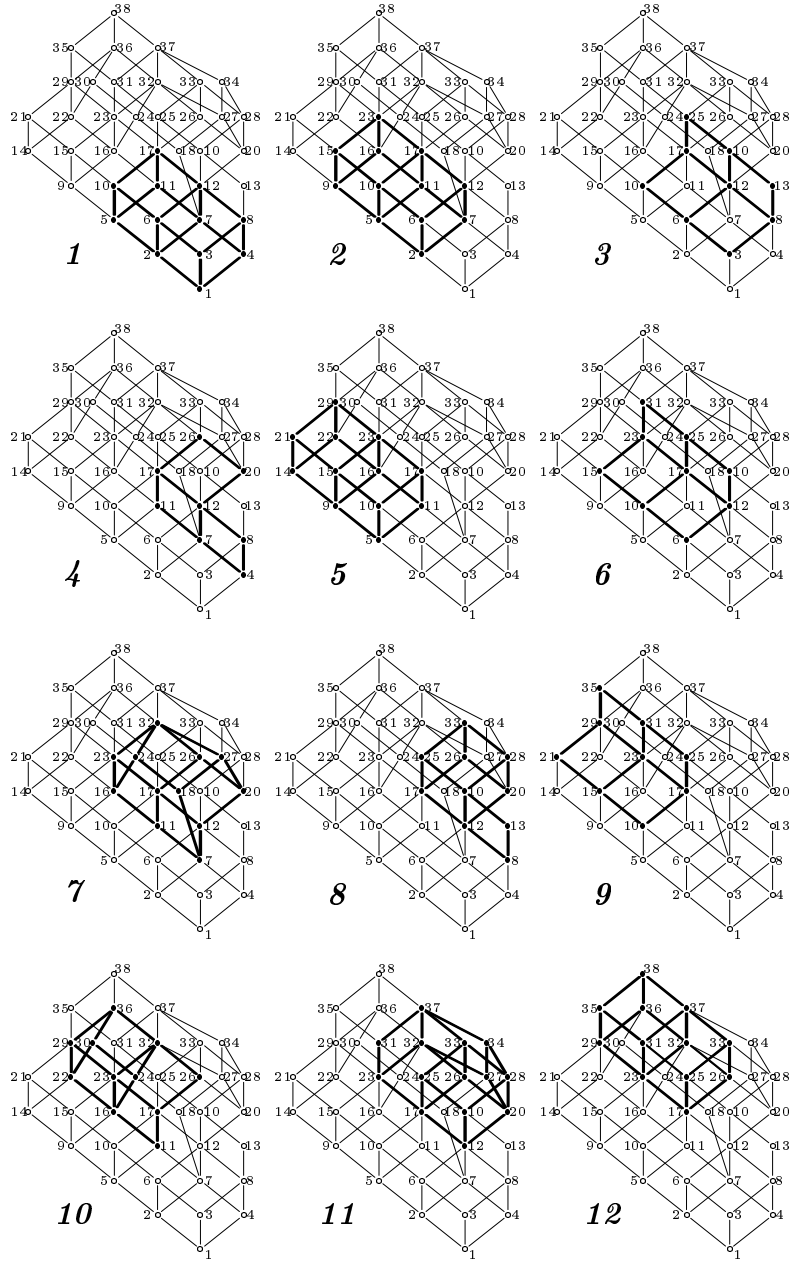
Figure 2: Blocks of the tolerance relation \frac{1}{2}E on the concept lattice of Fig. 1.
