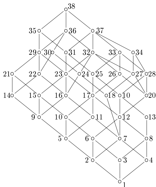
Figure 1: Concept lattice of the context in Tab. 1.
